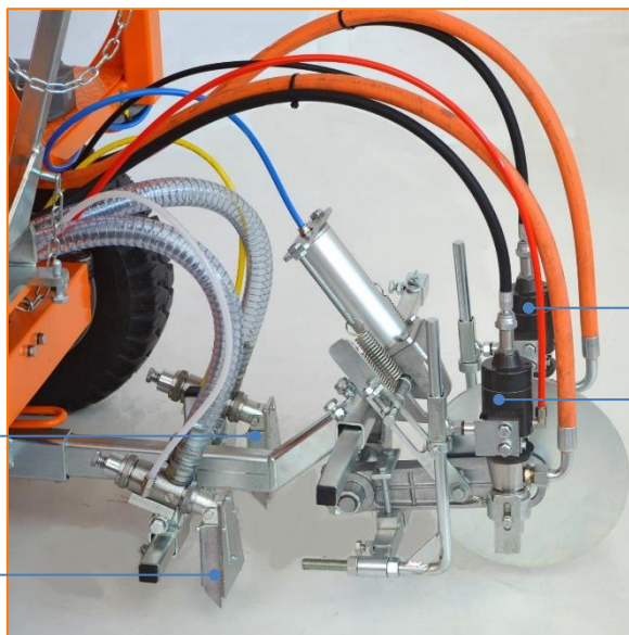
One-disc pneumatic support for paint gun (optional), mounted for central line
